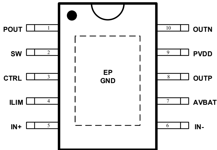
ESOP10(SPE) Top View
