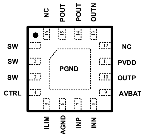
QFN3x3-16L(SQE) Top View
